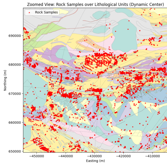
Figure 3. Zoomed view of rock samples (red) over lithological units, confirming correct spatial alignment of points and polygons prior to the spatial join.
