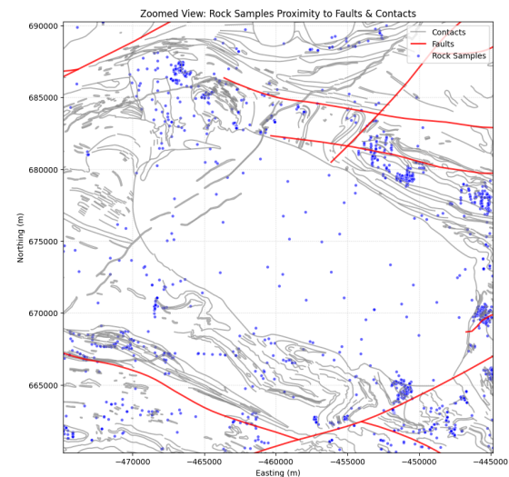
Figure 5. Local structural context — sample proximity to faults and contacts in a representative window, the scale at which the nearest-distance features are computed.
