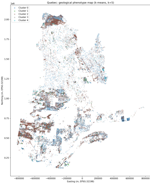
Figure 6. Spatial distribution of clusters.
